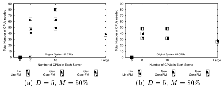
Fig. 3. Numbers of CPUs Required for Group 3
