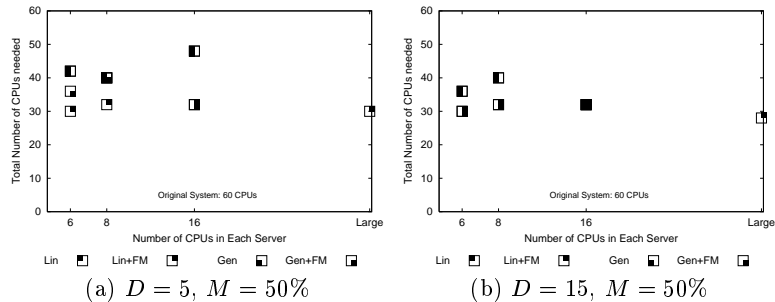
Fig. 2. Numbers of CPUs Required for Group 1
