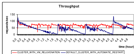
Figure 9: Comparing the cluster throughput, with and without rejuvenation, but automatic restart (Tomcat/Axis).
