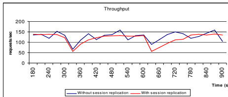
Figure 6: Comparing the overhead of session replication with session objects of 8kb (Tomcat/Axis).
