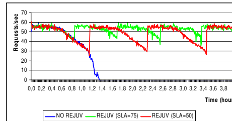
Figure 4: Applying Rejuvenation to TPC-W.
