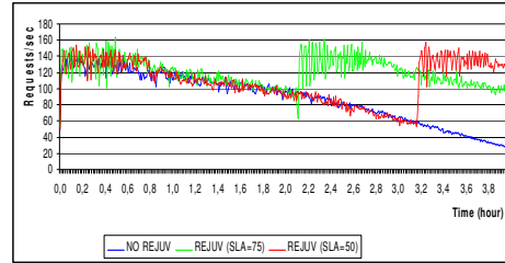
Figure 3: Applying Rejuvenation to Tomcat/Axis.
