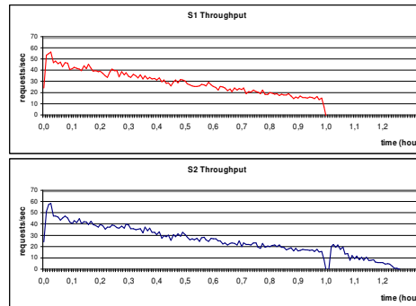
Figure 7: Throughput of two servers in a cluster, suffering from severe aging (Tomcat/Axis).
